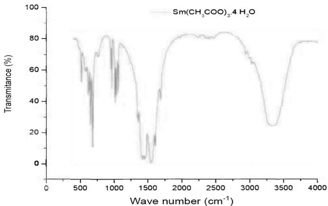
Figure 4: Infrared spectroscopy of the samarium acetate prepared [14]
