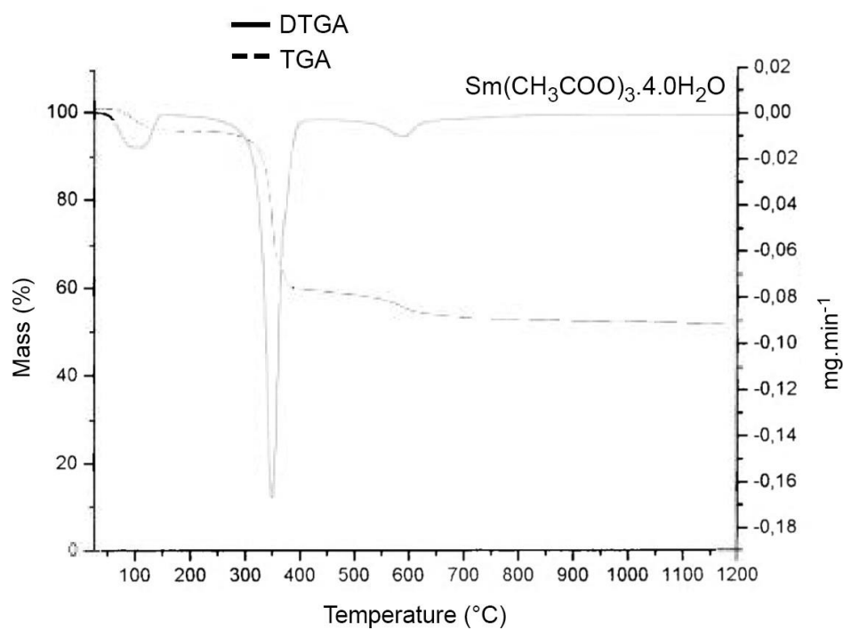
Figure 2: TG/ DTG of the samarium acetate prepared \text{Sm}(\text{CH}_3\text{COO})_3 \cdot 4.0\text{H}_2\text{O}
