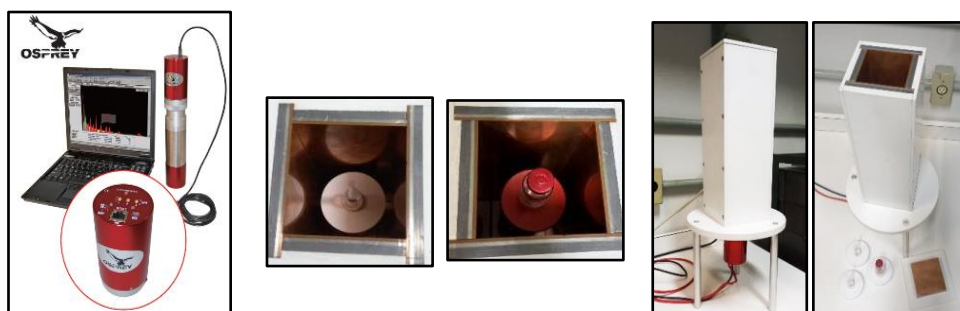
Figure 1: Arrangement of the gamma spectrometry system with NaI(Tl), containing the detector crystal, associated electronics, source holder, and lead shielding.
