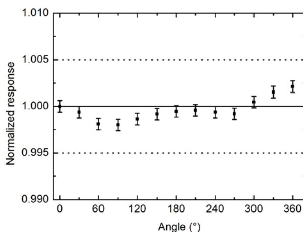
Figure 4: Angular dependence test of the new graphite ionization chamber developed at the IPEN. The dashed lines represent the recommended limits of \pm 0.5\% [8]
