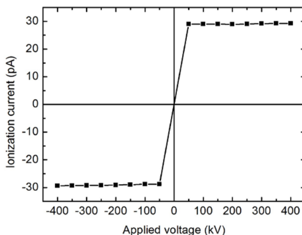
Figure 2: Saturation curves of the new graphite ionization chamber developed at the IPEN for ^{60}\text{Co} beams. The maximum uncertainty was 0.1%, and therefore not visible in the figure
