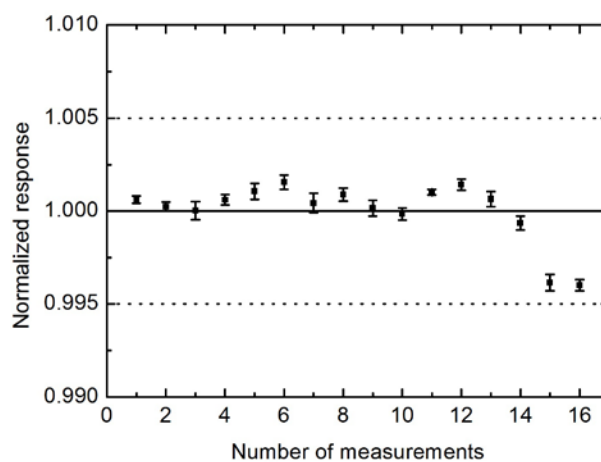
Figure 3: Medium-term stability test of the new graphite ionization chamber developed at the IPEN. The dashed lines represent the recommended limit of \pm 0.5\% [8]
