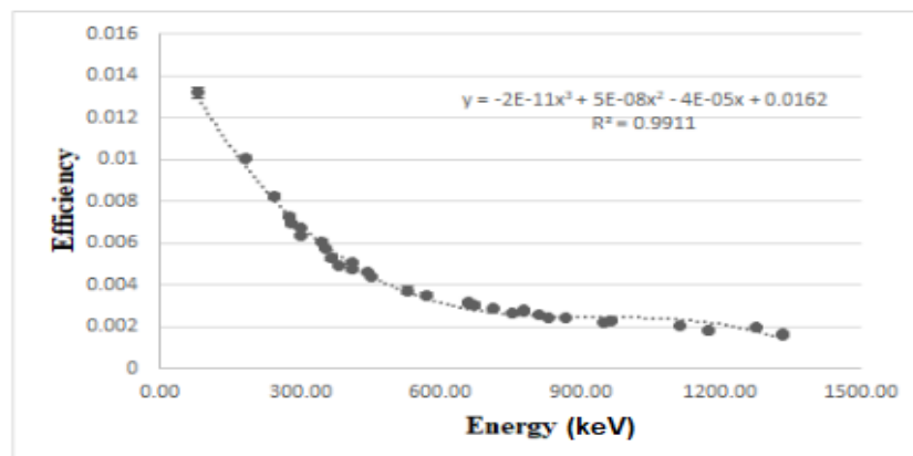
Figure 1: Efficiency curve as a function of energy, obtained for the HPGe detector at 100 mm distance source-detector.
