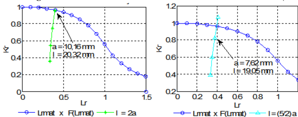
Figure 6 - External axial crack – Level 2 - normal assessment of R6 (Matlab)
