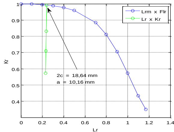
Figure 4 - External axial (longitudinal) crack – Level 2 assessment of BS-7910 obtained in Matlab
