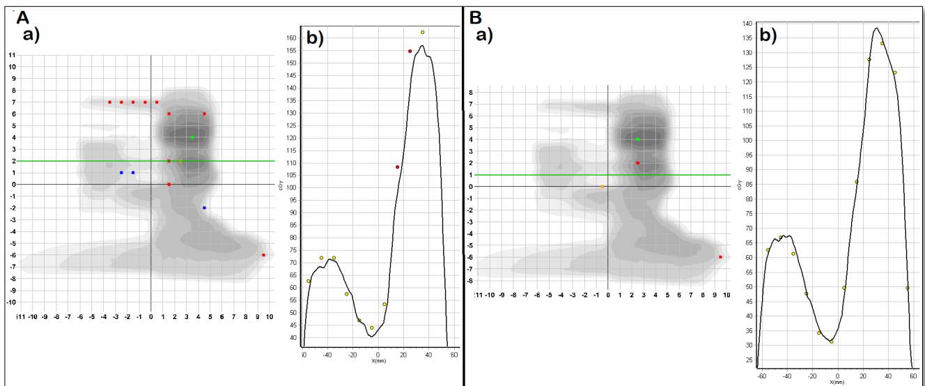
Figure 7: Gamma analysis for the HDMLC field calculated with the geometric modeling parameters provided by the manufacturer (A) and after post modeling (B). In a) example of dose fluency measured on the X axis (green line), where the dose profile from figure b) was removed and this highlights the discrepancy between the measured (curve dotted) and calculated doses (continue curve).
