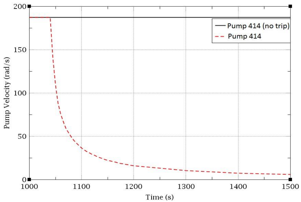
Figure 7: Pump 414 Velocity Evolution.
