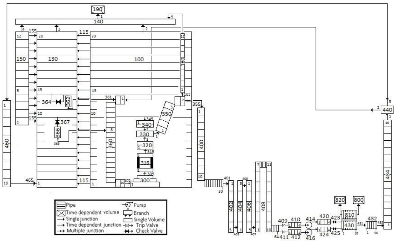
Figure 3: RMB nodalization for RELAP5/Mod3 (adapted from [17]).
