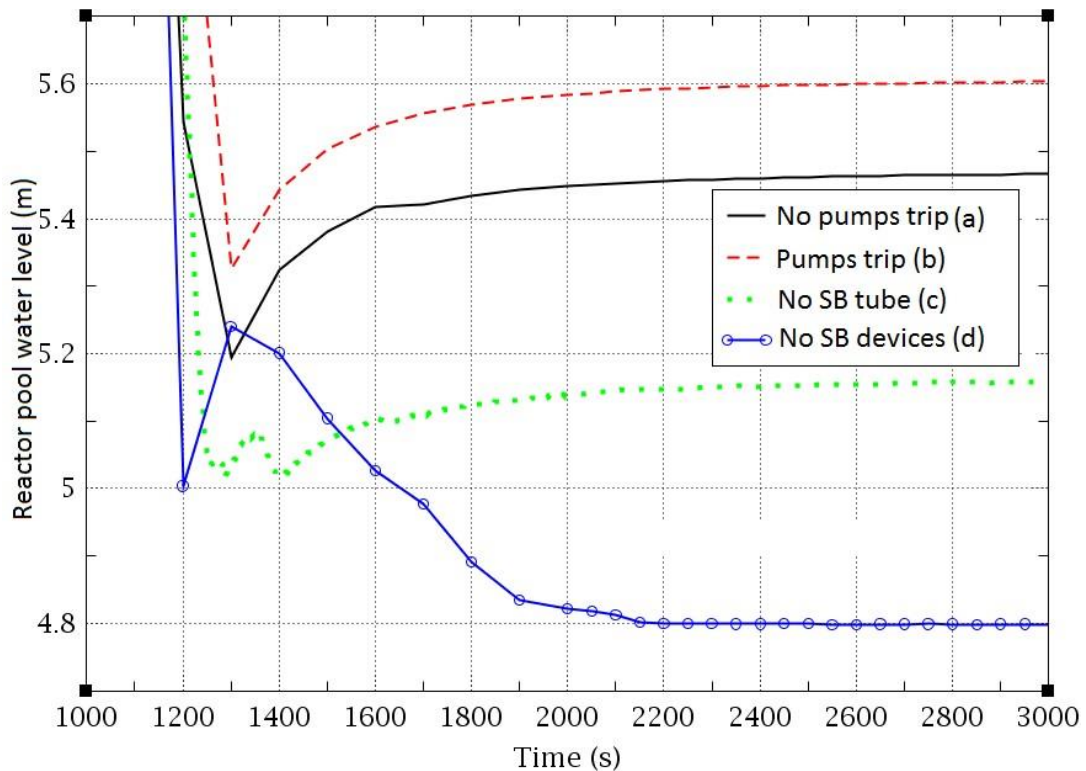
Figure 10: Reactor Pool Water Level Evolution.
