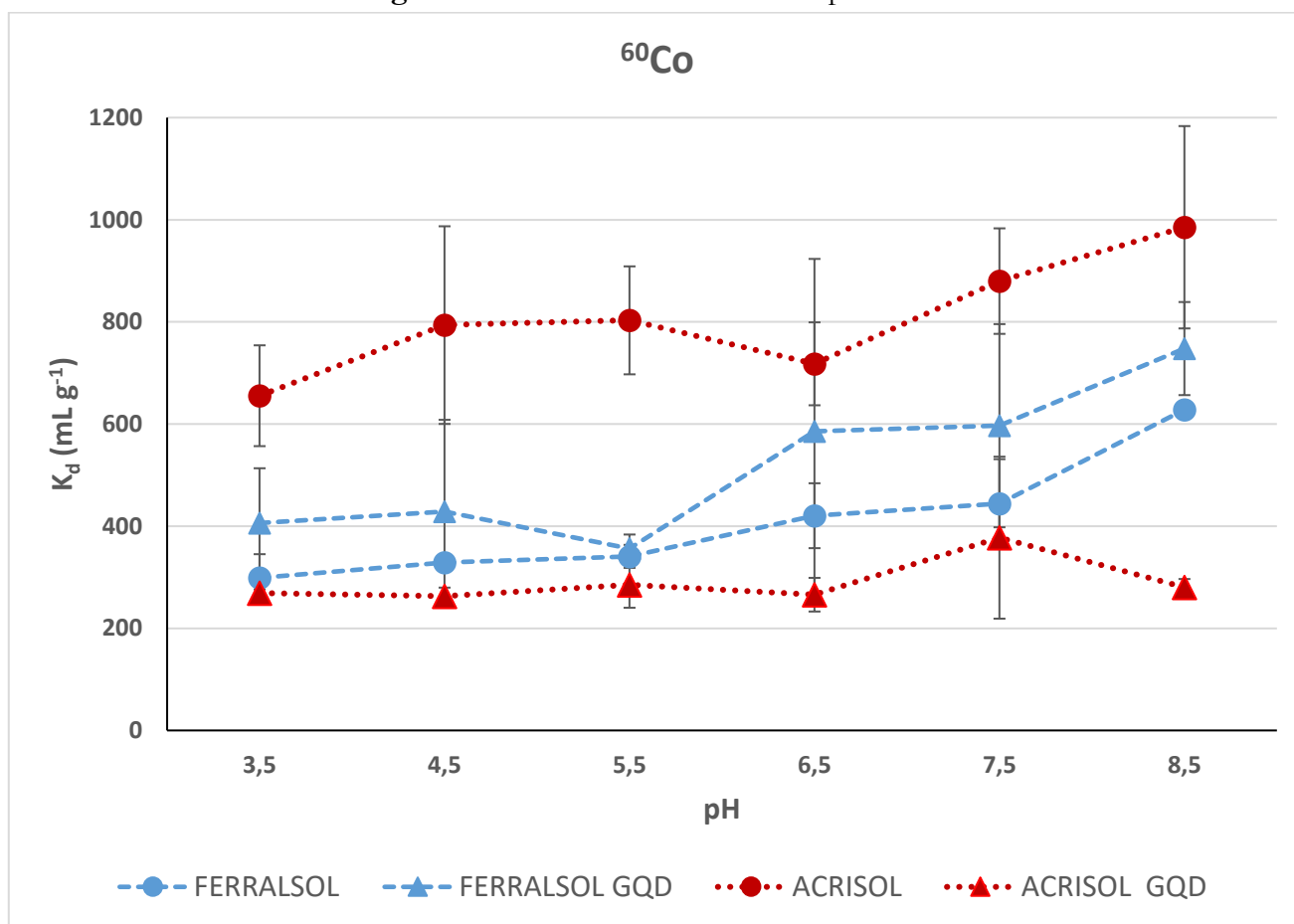
Figure 2: ^{60}\text{Co} Kd values at different pH values
