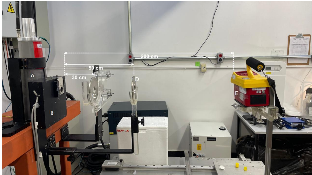
Figure 1: Experimental arrangement, where there is the x-ray tube (A), the shutter (B), the first collimator (C), the second collimator (D), and the ionization chamber (E).
