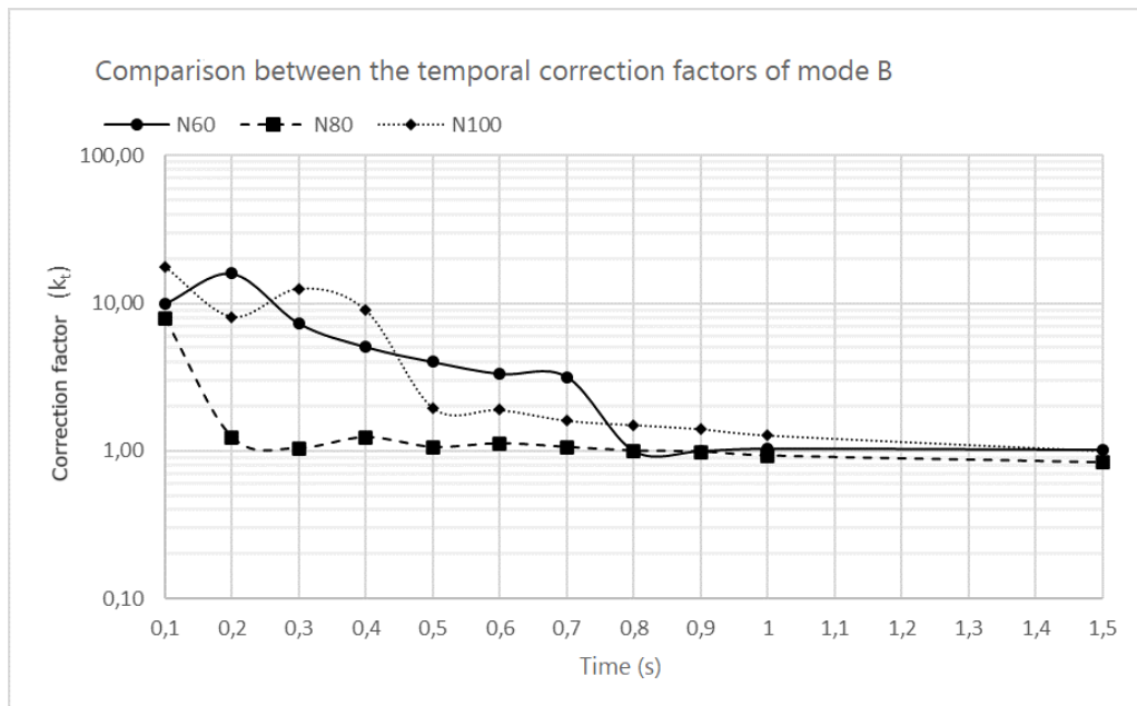
Figure 9: Comparative graph of the correction factors for N60, N80, and N100 in mode B.
