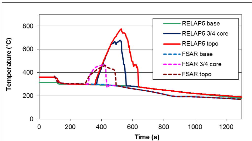
Figure 12: Hot rod cladding temperature of ANGRA 2 core.
