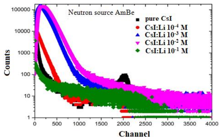
Figure 11: Detection spectra obtained with CsI:Li and pure CsI crystals excited with neutron radiation from a AmBe source.
