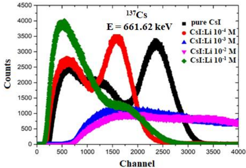
Figure 9: Detection spectra obtained with CsI:Li and pure CsI crystals excited with gamma radiation from a ^{137}\text{Cs} .
