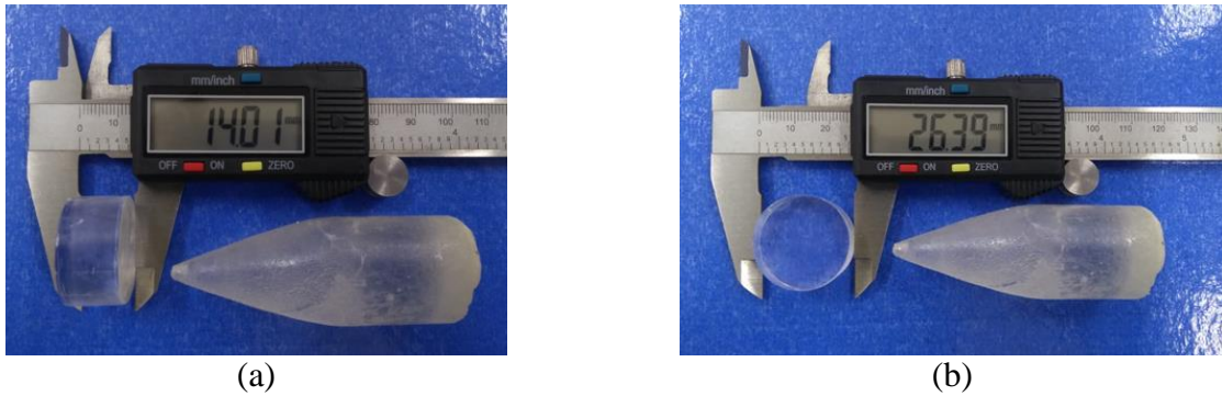
Figure 3: Scintillator crystal CsI:Li 10^{-3} M. (a) cut crystal in the geometry adopted for this work (b) polished crystal and crystal in the geometric shape of the crucible.
