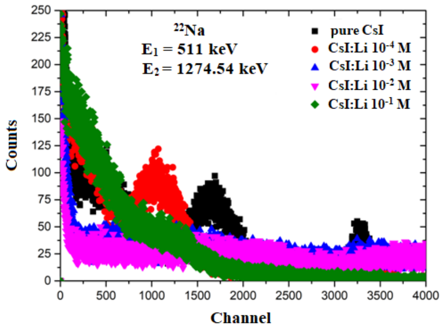
Figure 8: Detection spectra obtained with CsI:Li and pure CsI crystals excited with gamma radiation from a ^{22}\text{Na} source.
