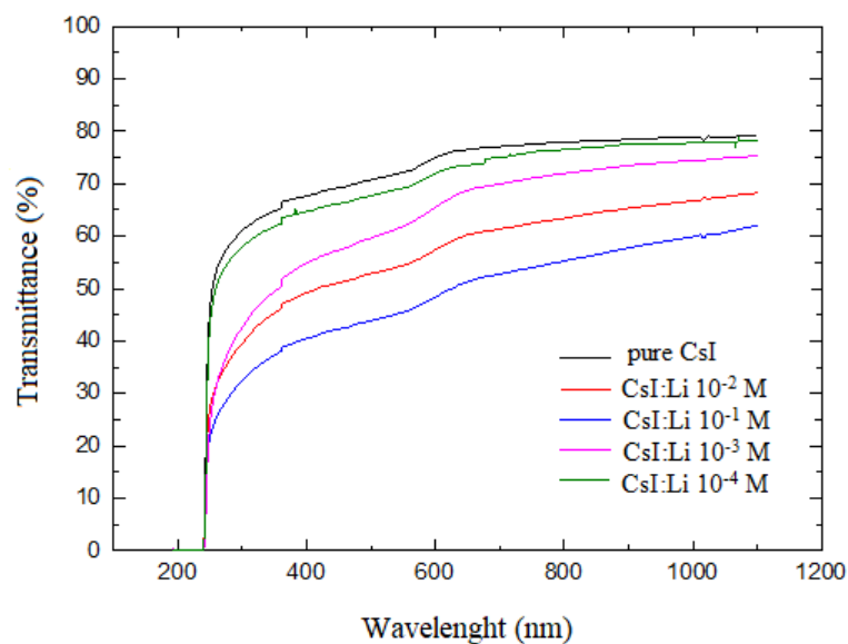
Figure 4: Transmittance curves as a function of wavelength for pure CsI and CsI:Li crystals with thicknesses of 3 mm.
