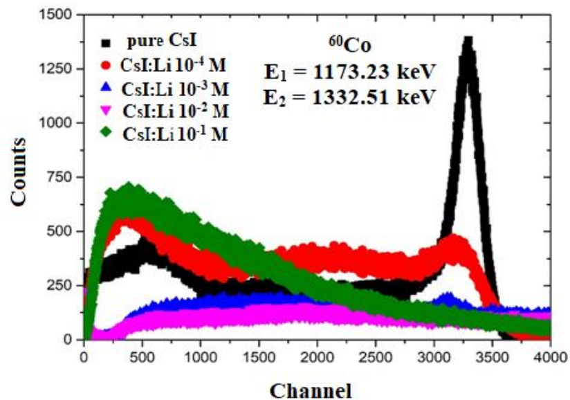
Figure 10: Detection spectra obtained with CsI:Li and pure CsI crystals excited with gamma radiation from a ^{60}\text{Co} source.
