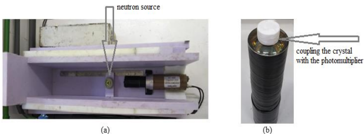
Figure 2: Assembled arrangement for neutron measurement, which is formed by a borated polystyrene barrier and paraffin plates (a) and the scintillator crystal optically coupled to the photomultiplier tube (b).
